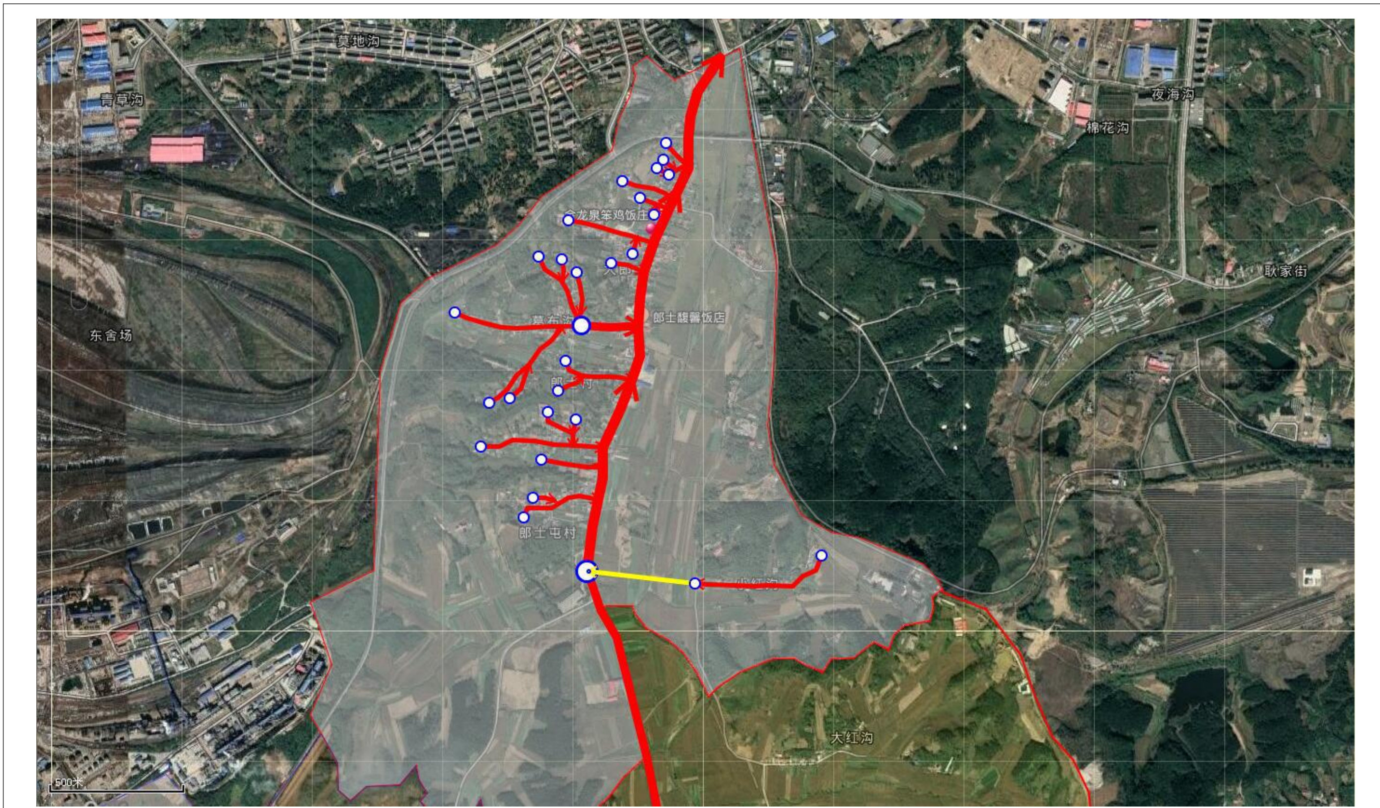
附图3 郎士村污水管网规划
